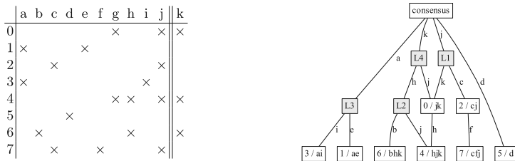
Fig. 1. (Left) A data table of genetic variations for individuals of a particular population. (Right) A median graph for the data table.
