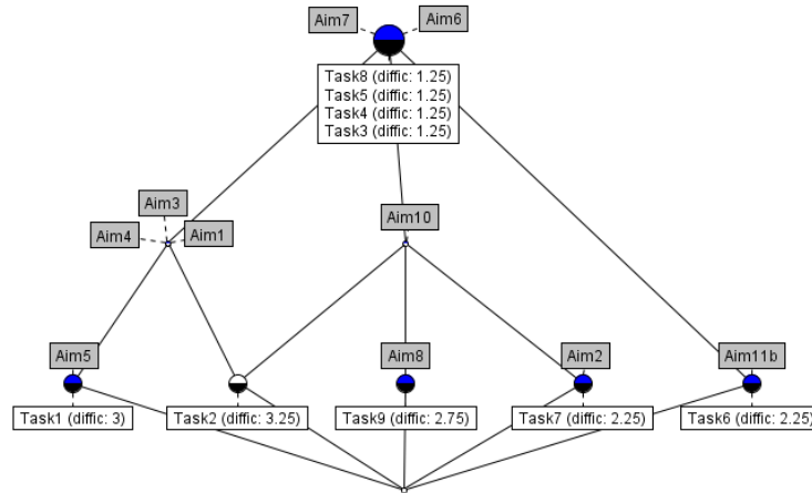
Fig. 2. Concept lattice of the participated teacher
