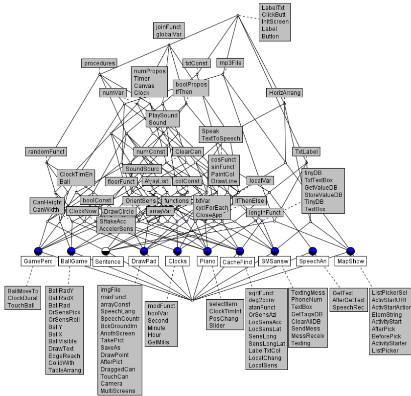
Fig. 5. A concept lattice of App Inventor 2 programming in education
